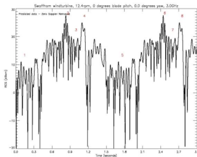
Figure 4-5: The Swaffham turbine RCS versus time at 0° pitch, 0° yaw, with the zero-Doppler component removed.
