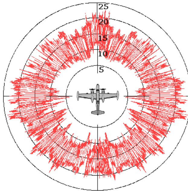
RCS-waarden in dB square meter (dBsqm)
