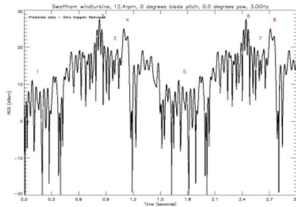
Figure 4-5: The Swaffham turbine RCS versus time at 0^\circ pitch, 0^\circ yaw, with the zero-Doppler component removed.
