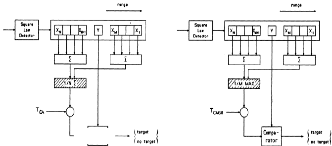
Fig. 2. Comparison of CA and CAGO CFAR procedures.
