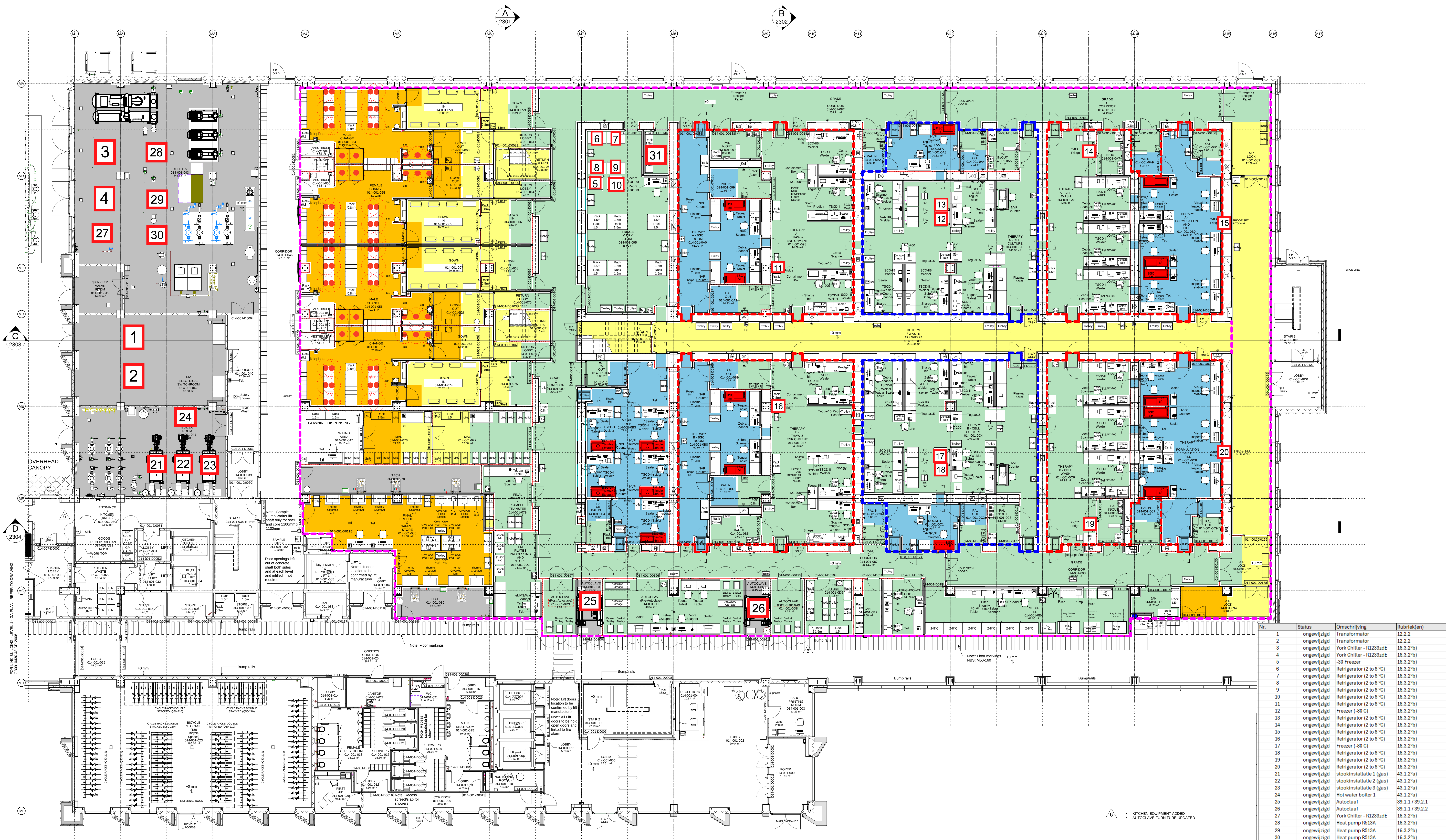
GA PLAN - GROUND FLOOR 1 : 100
