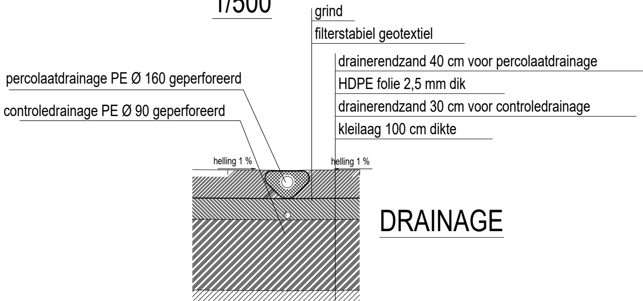
DETAIL DEPONIE IV 1/500
