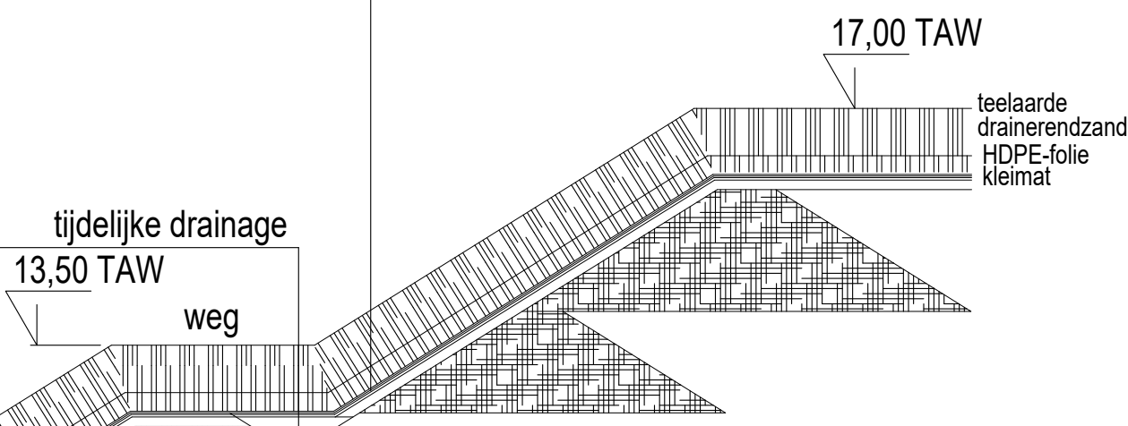
DETAIL DEPONIE IV 1/1000
