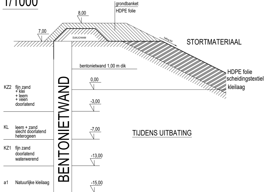
DETAIL DEPONIE IV 1/1000
