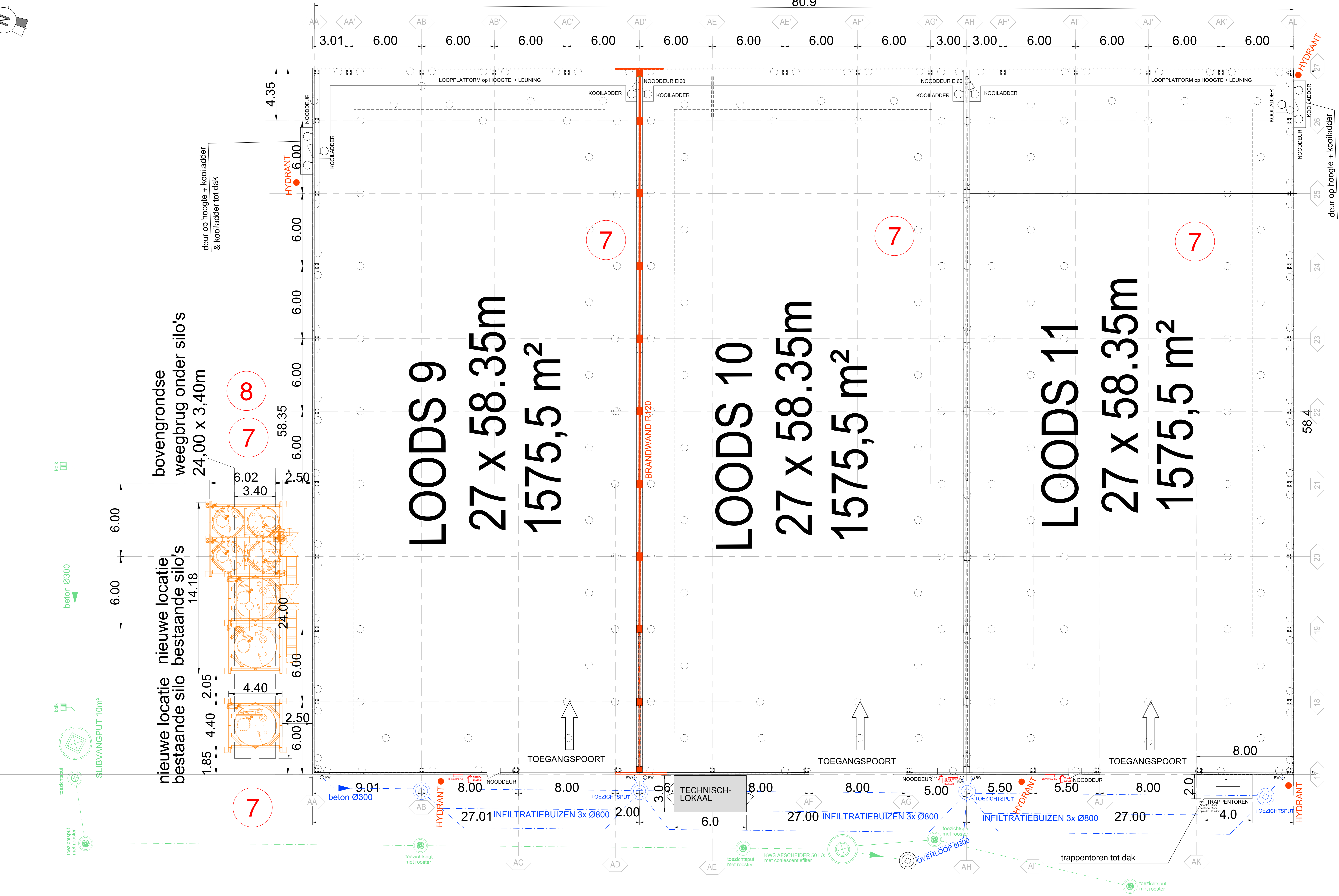
RIOLERINGSPLAN LOODS 9-11
