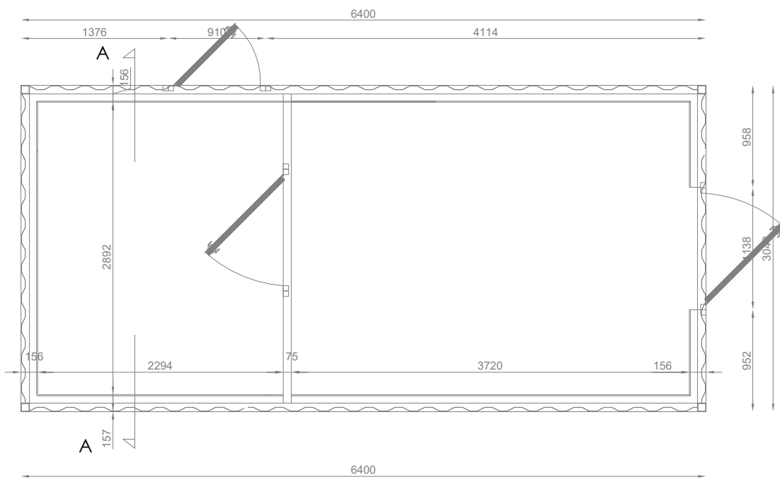
PLAN CONTROLEKAMER
