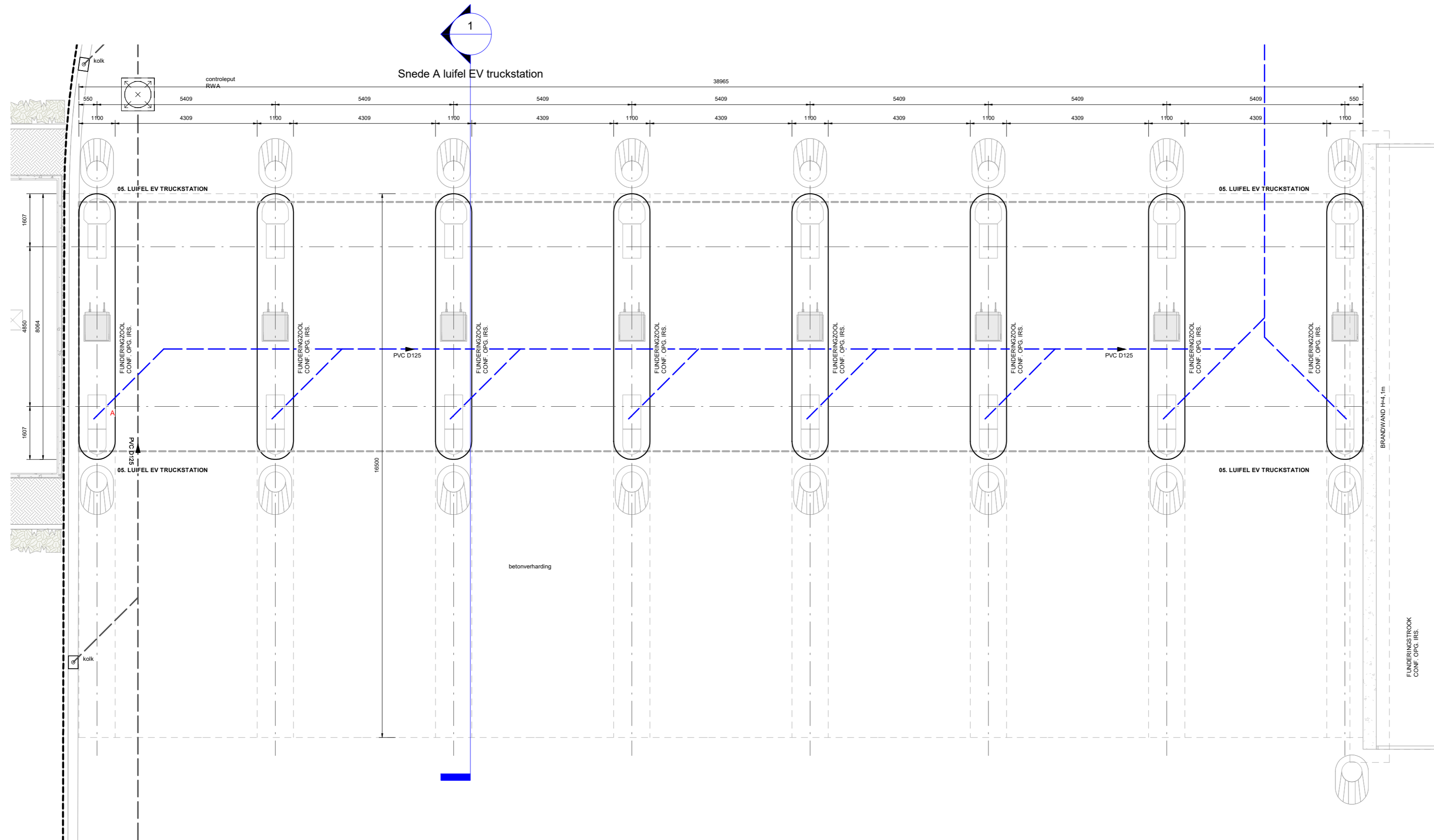
1 Fundering luifel EV truckstation 1 : 100
