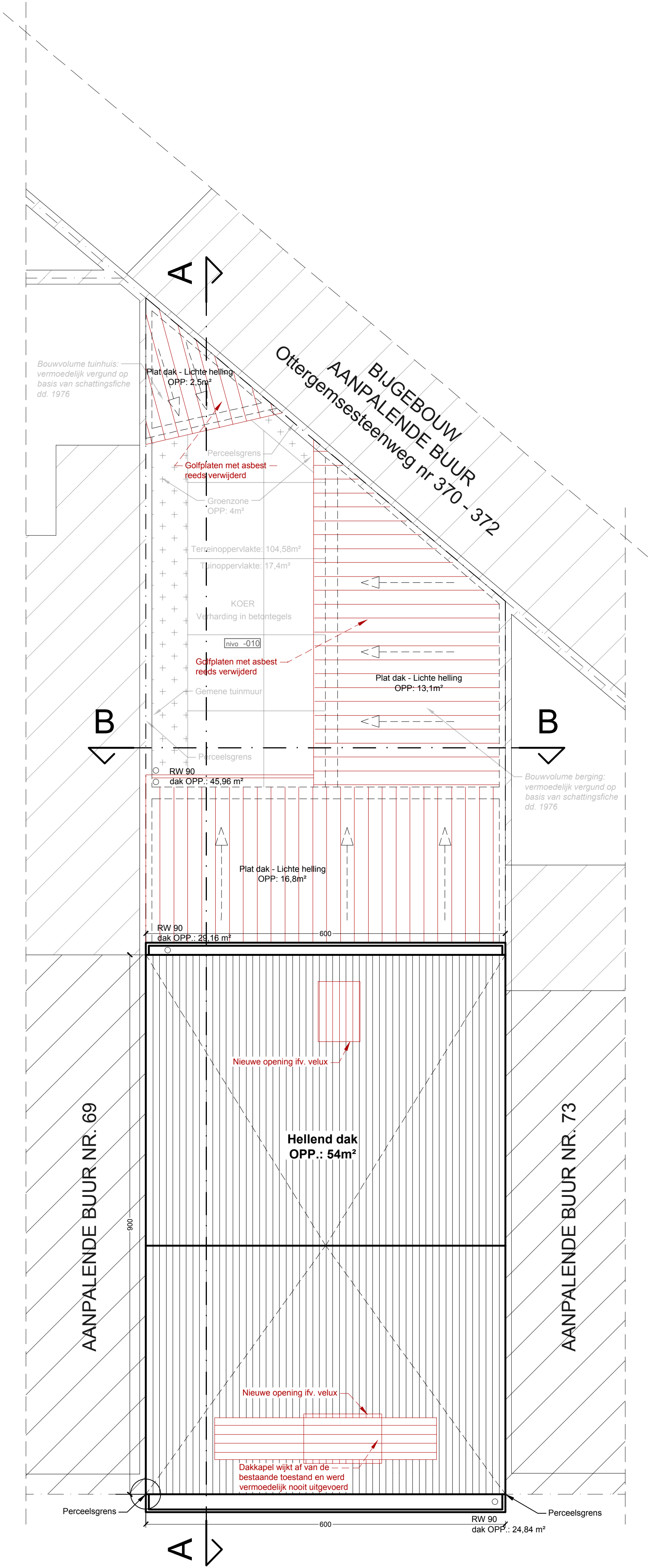
Dakenplan - vergund
