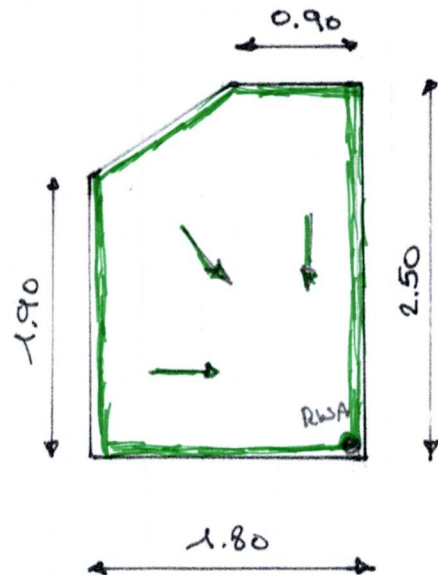
DAK PLAN
