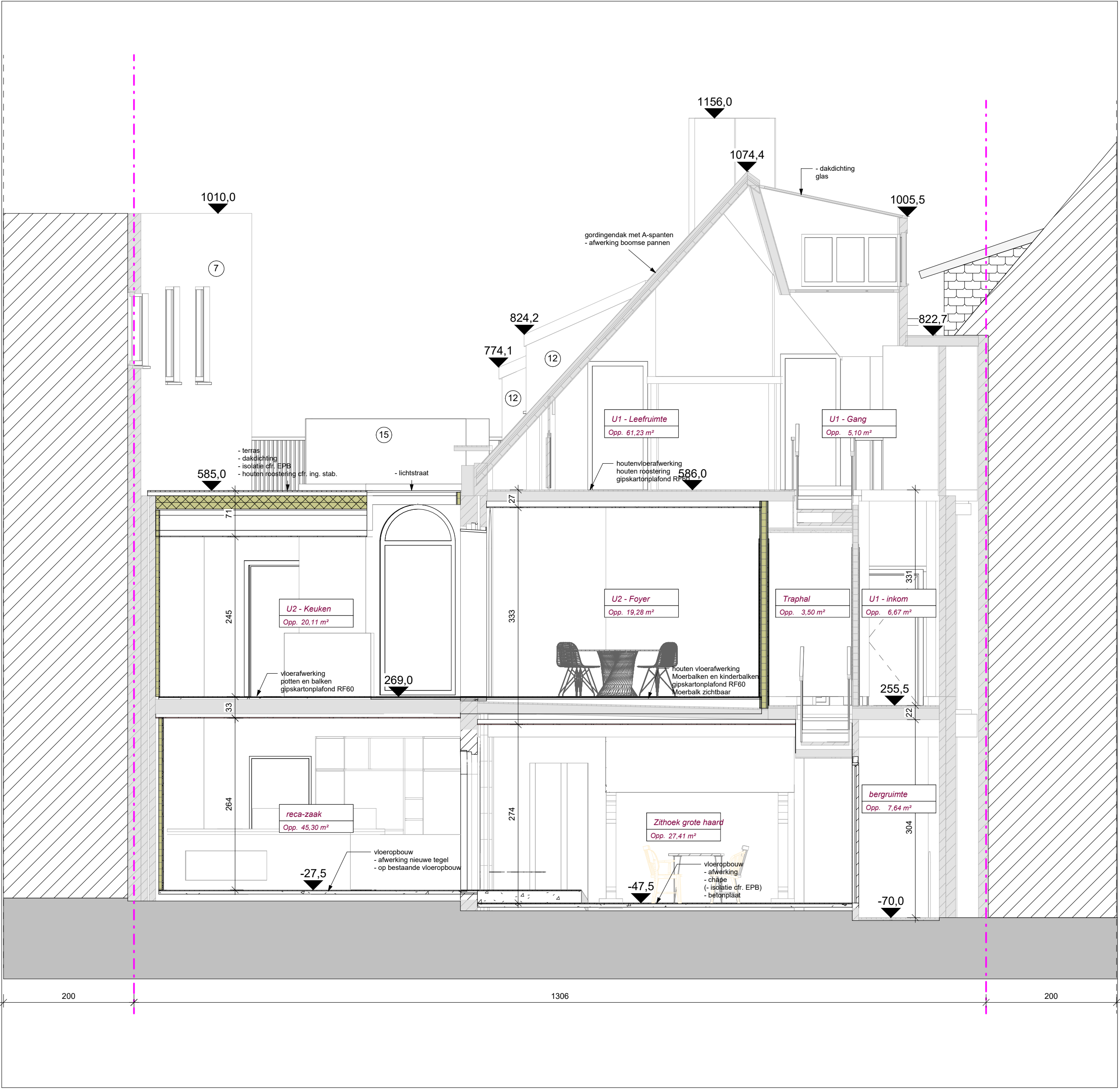
BA_3.01_X S_N_3.01_Dwarsdoorsnede
