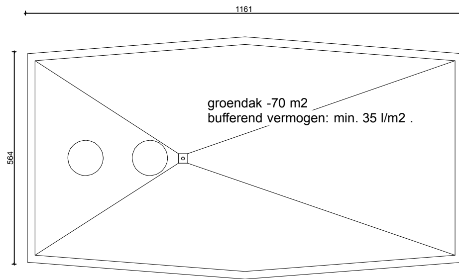
dakplan
