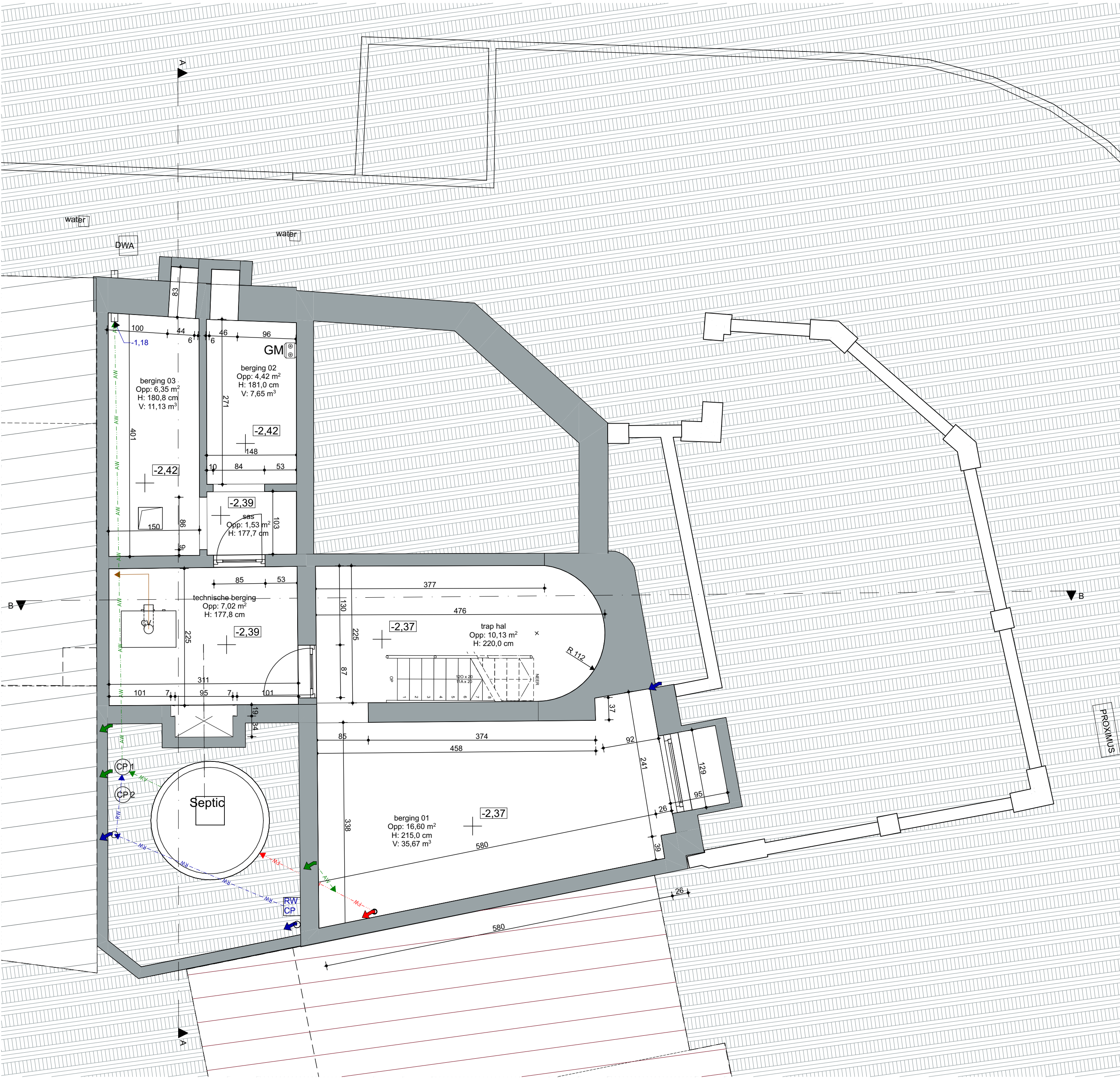
-1. Fundering 1:50
