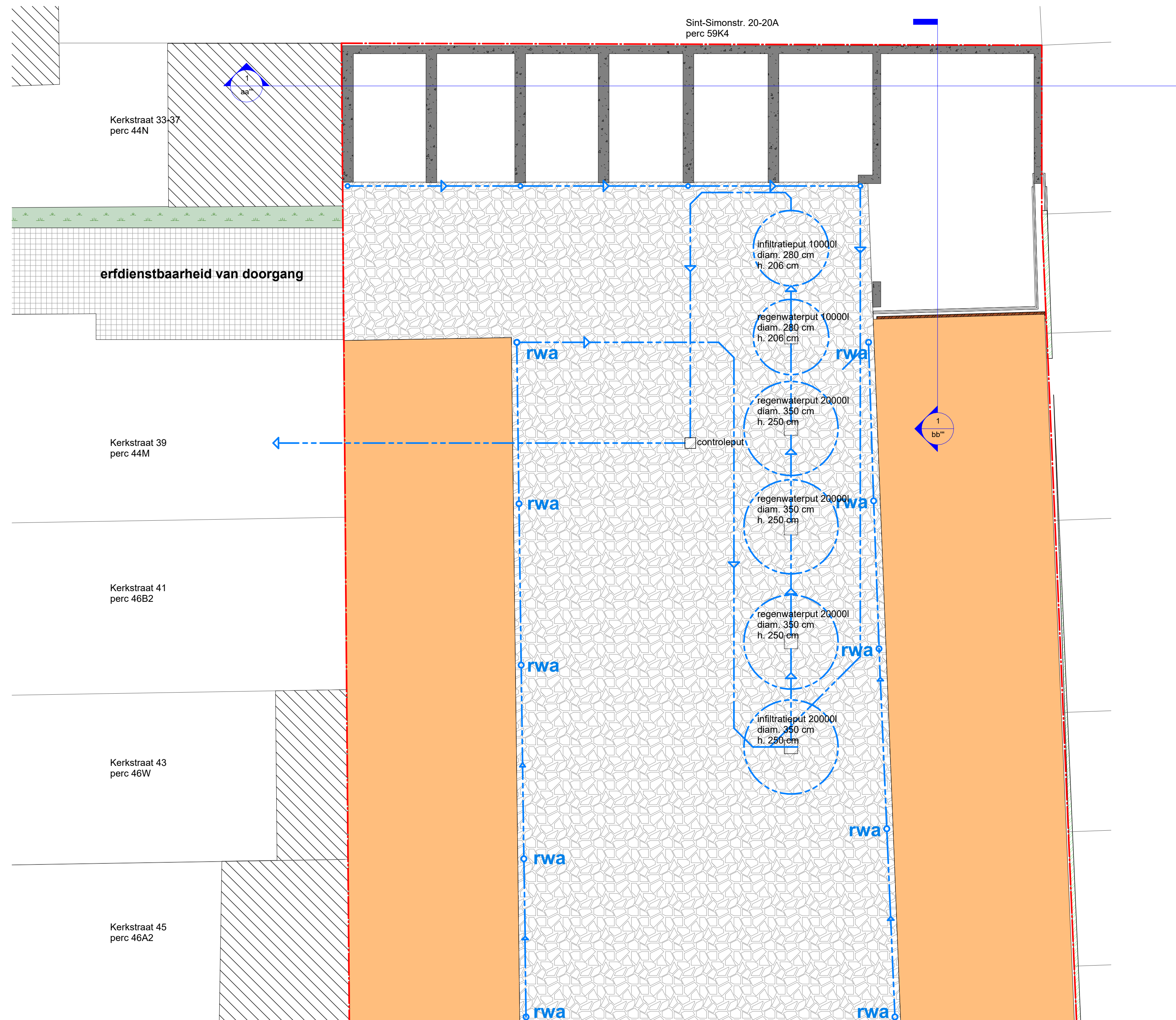
1 BA_garageboxen_P_N_-05_fundering & riolering 1 : 100
