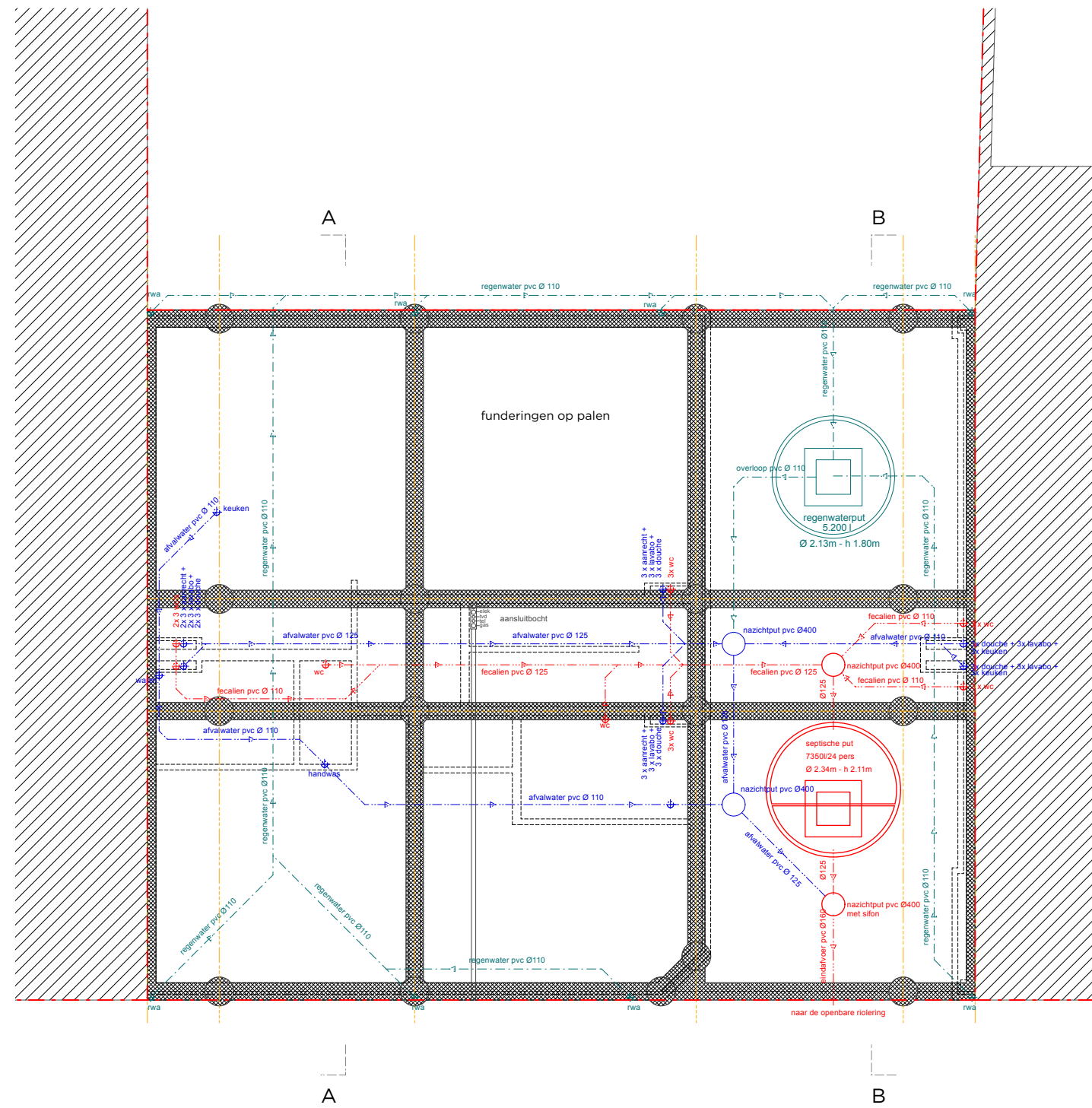
FUNDERINGEN - RIOLERING
