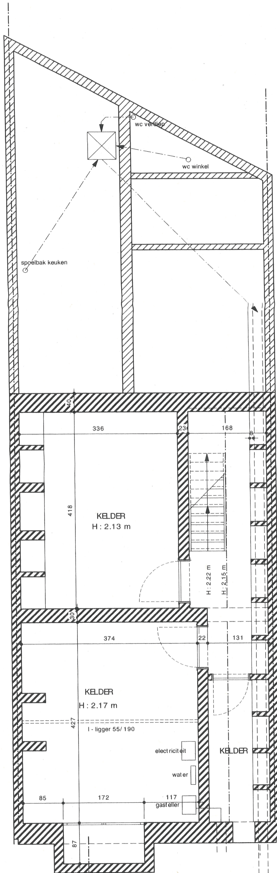
KELDER-EN RIJLINGSPLAN
