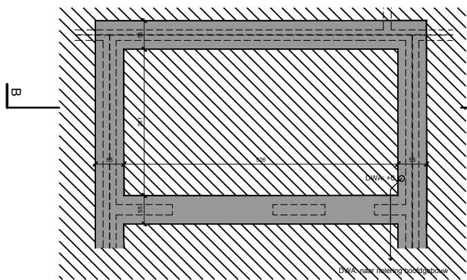
RIOLERINGSPLAN / 1:100
