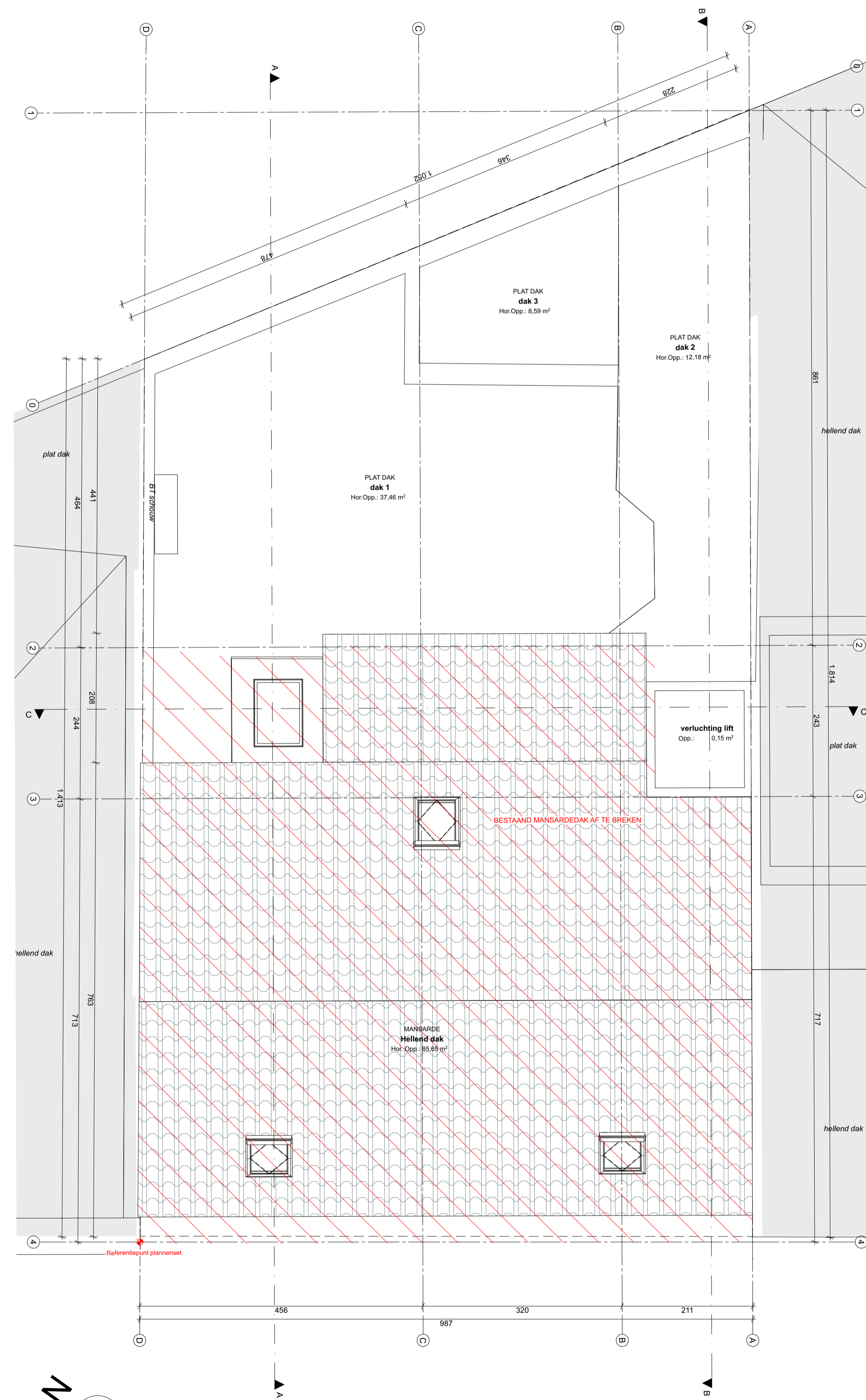
BT - DAKENPLAN
