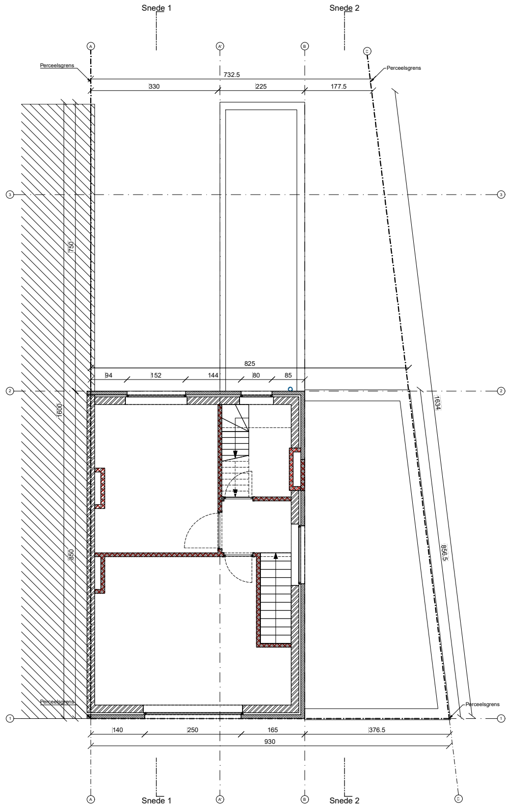
Grondplan +1
