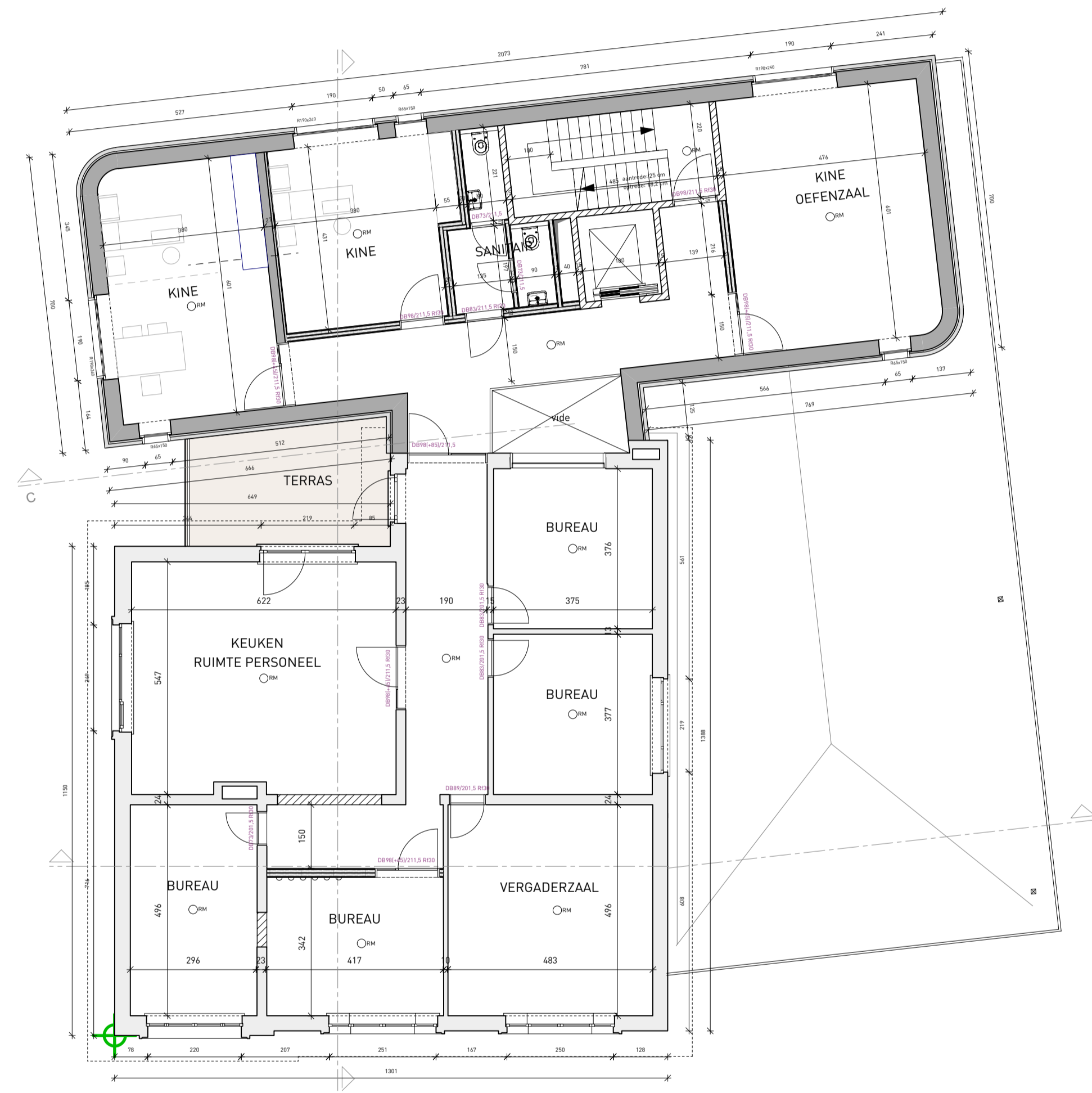
PLAN VERDIEPING
