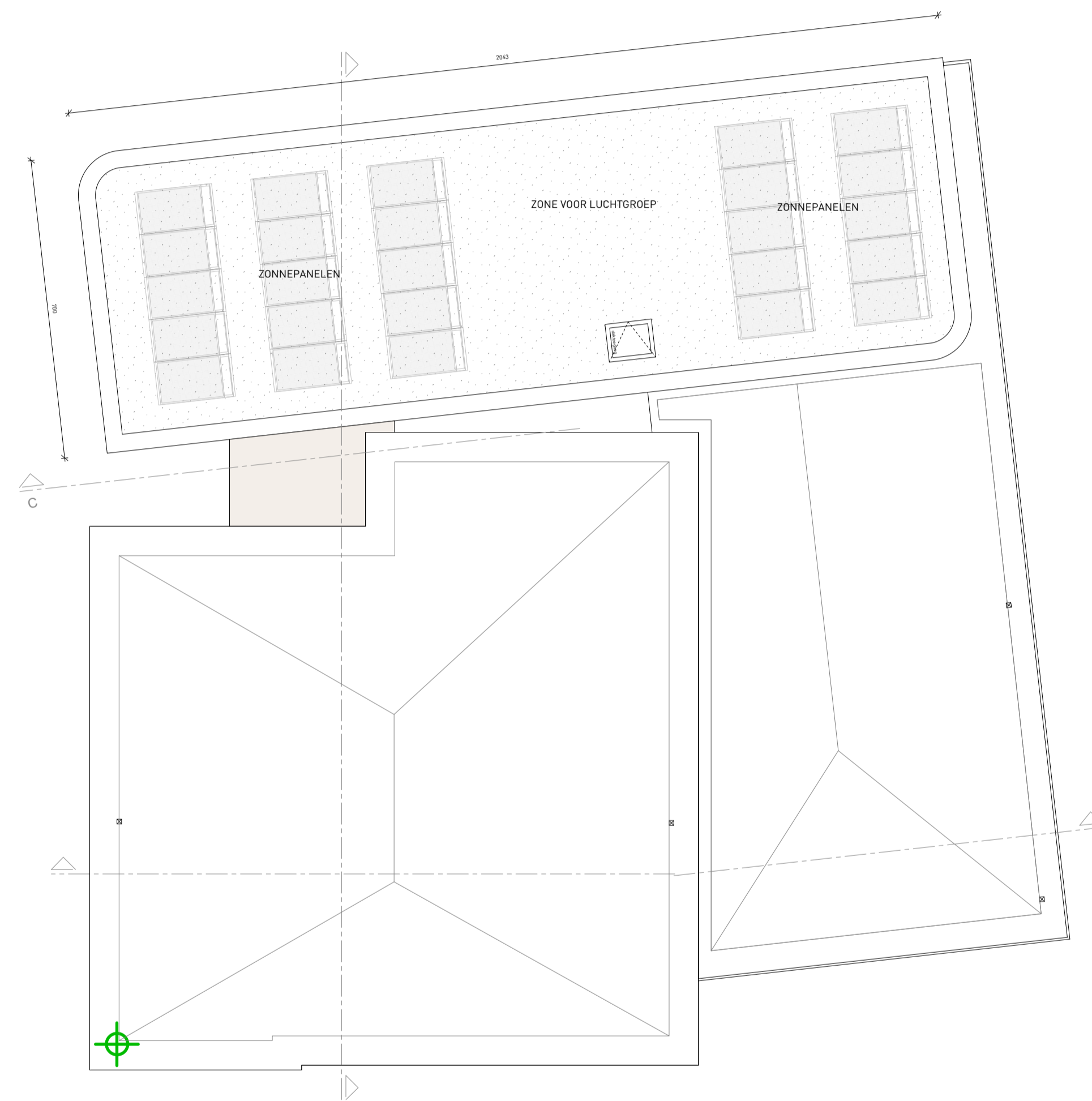
PLAN VERDIEPING
