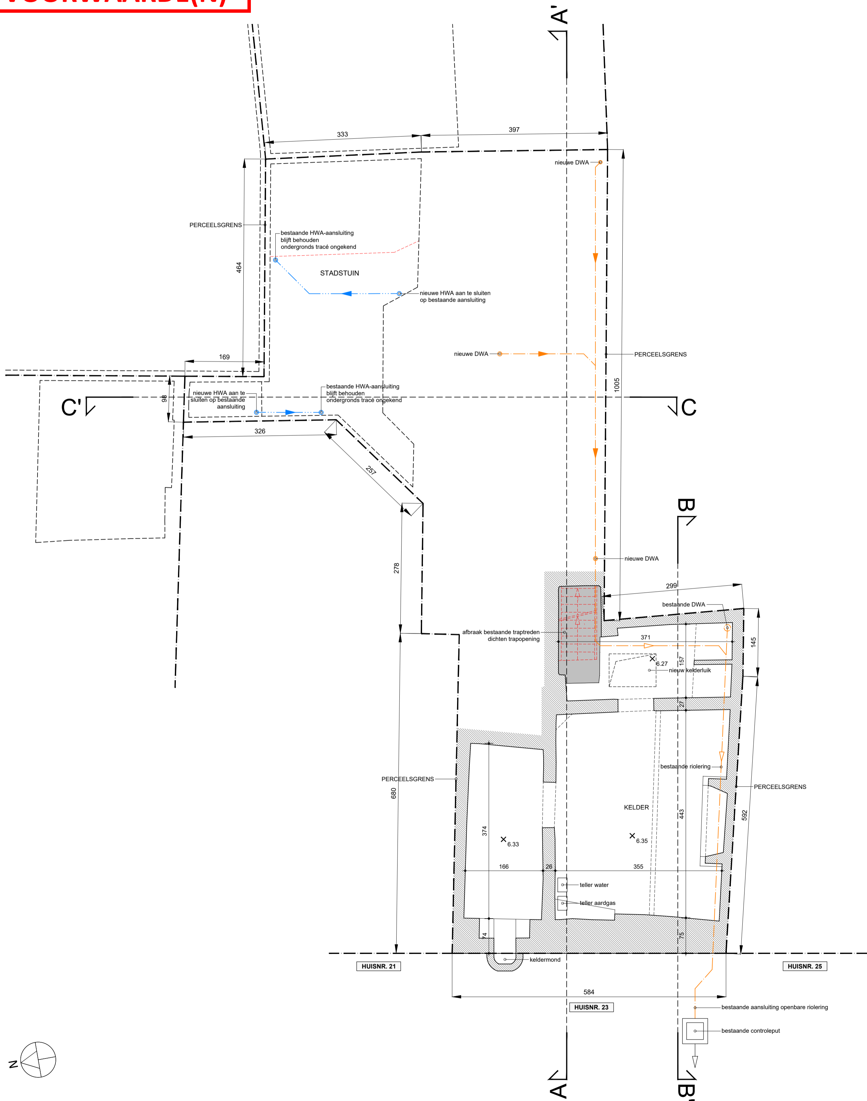
KELDERPLAN - RIOLERING
