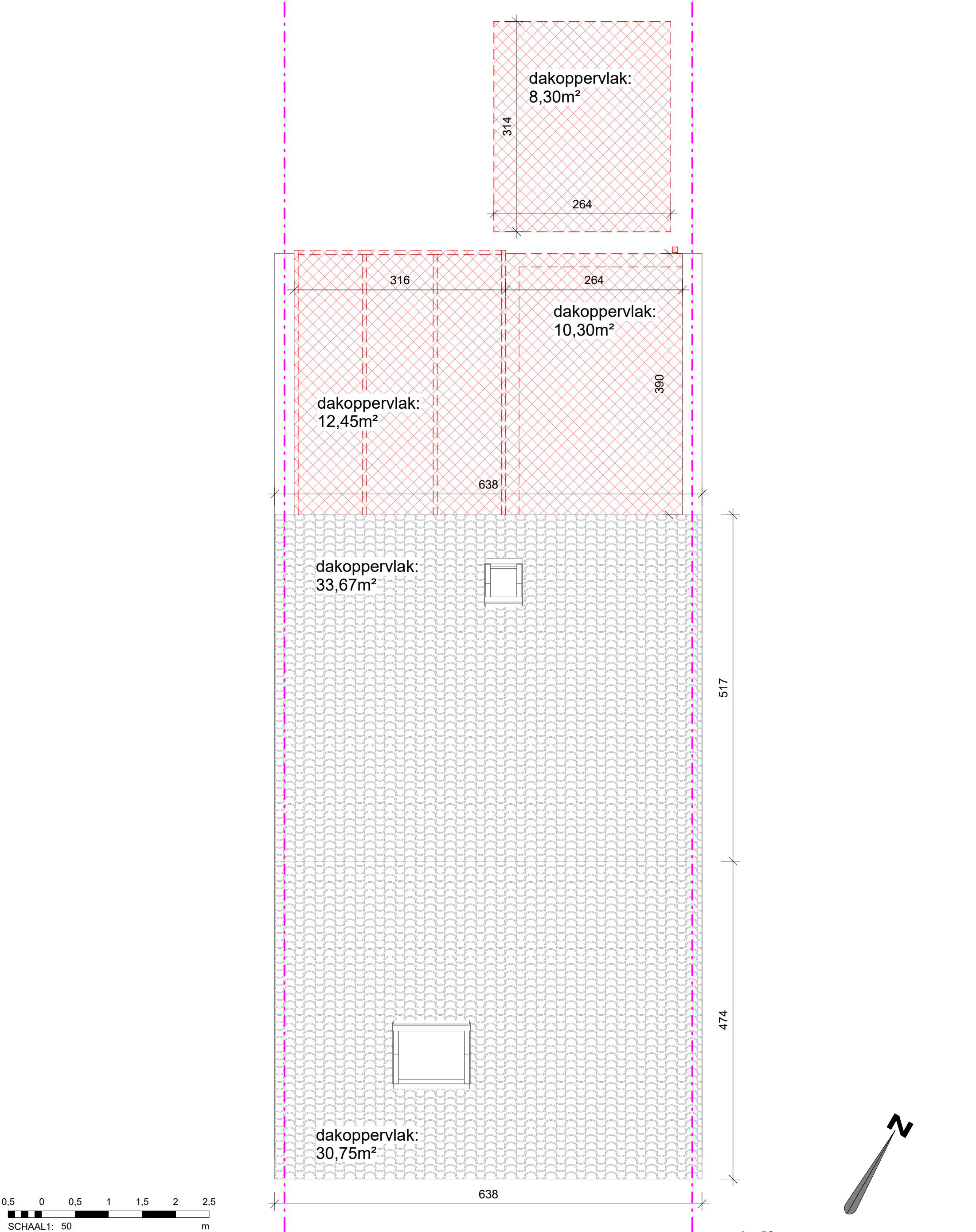
BA_1.30 P_B_1.30_Dakenplan
