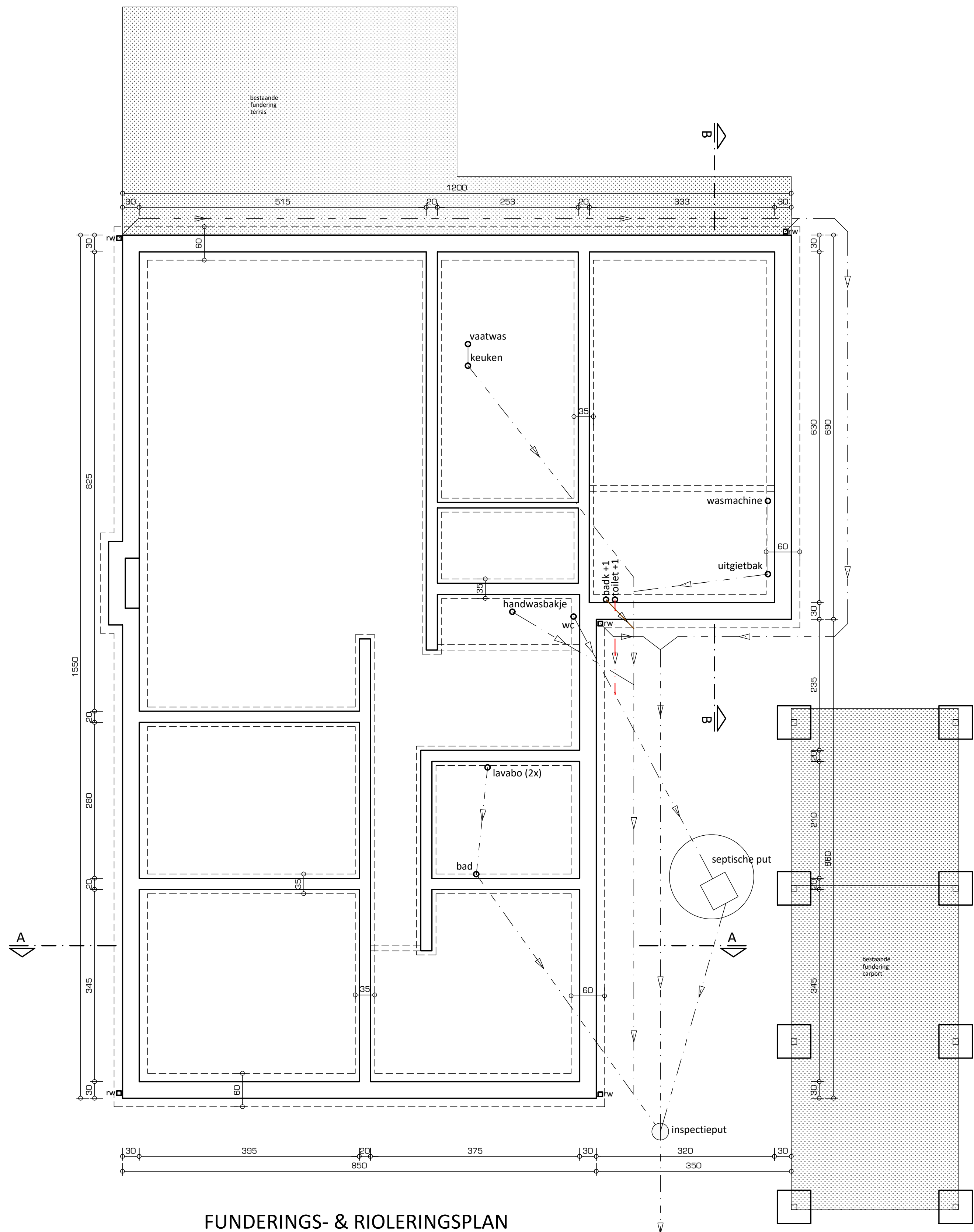
FUNDERINGS- & RIOLERINGSPLAN
