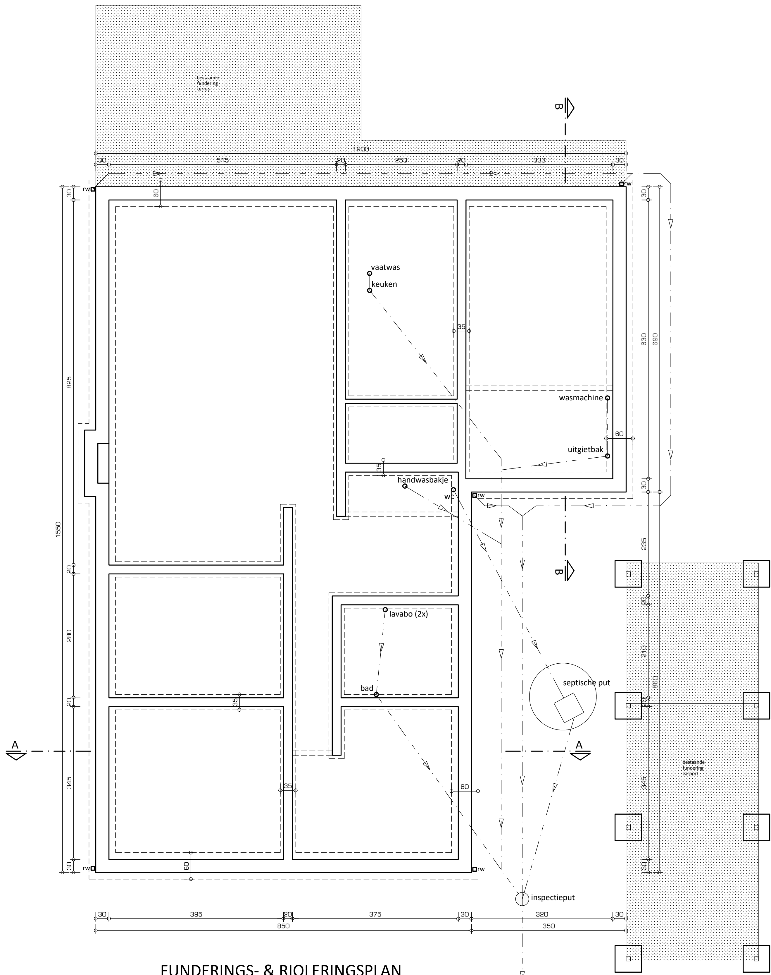
FUNDERINGS- & RIOLERINGSPLAN
