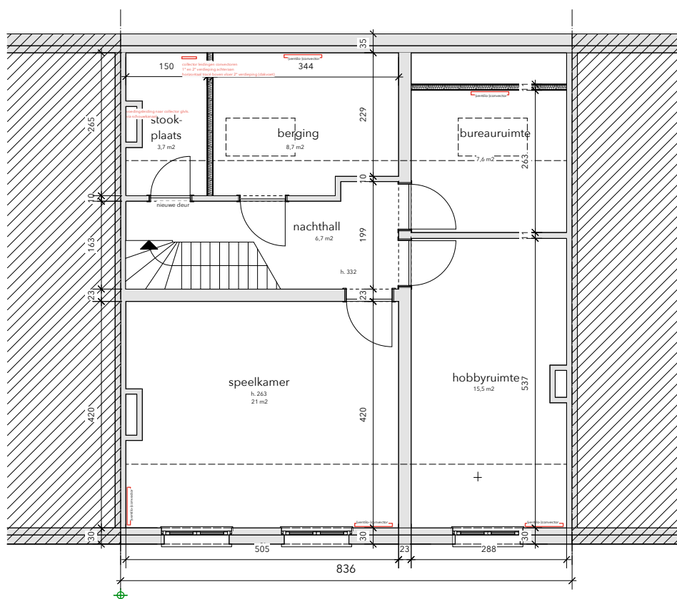
plan v.d. dakverdieping
