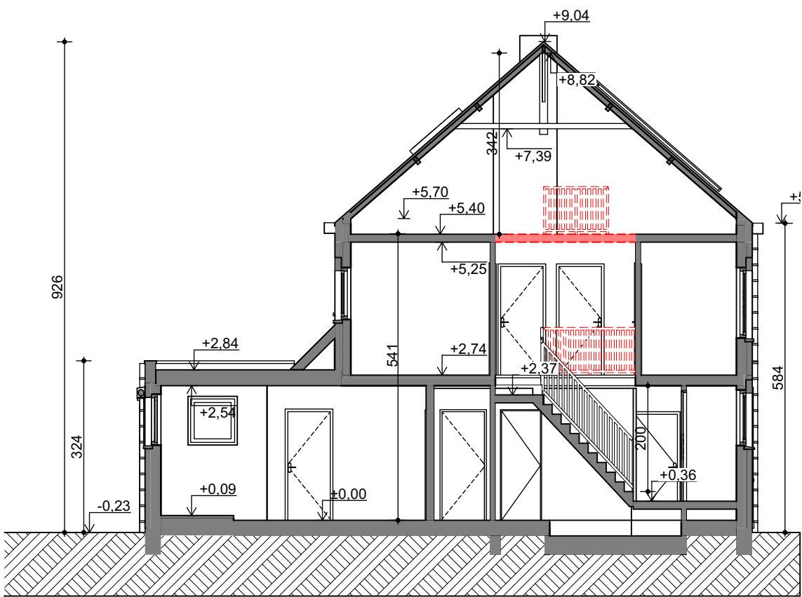
S_B Doorsnede B-B 1:100
