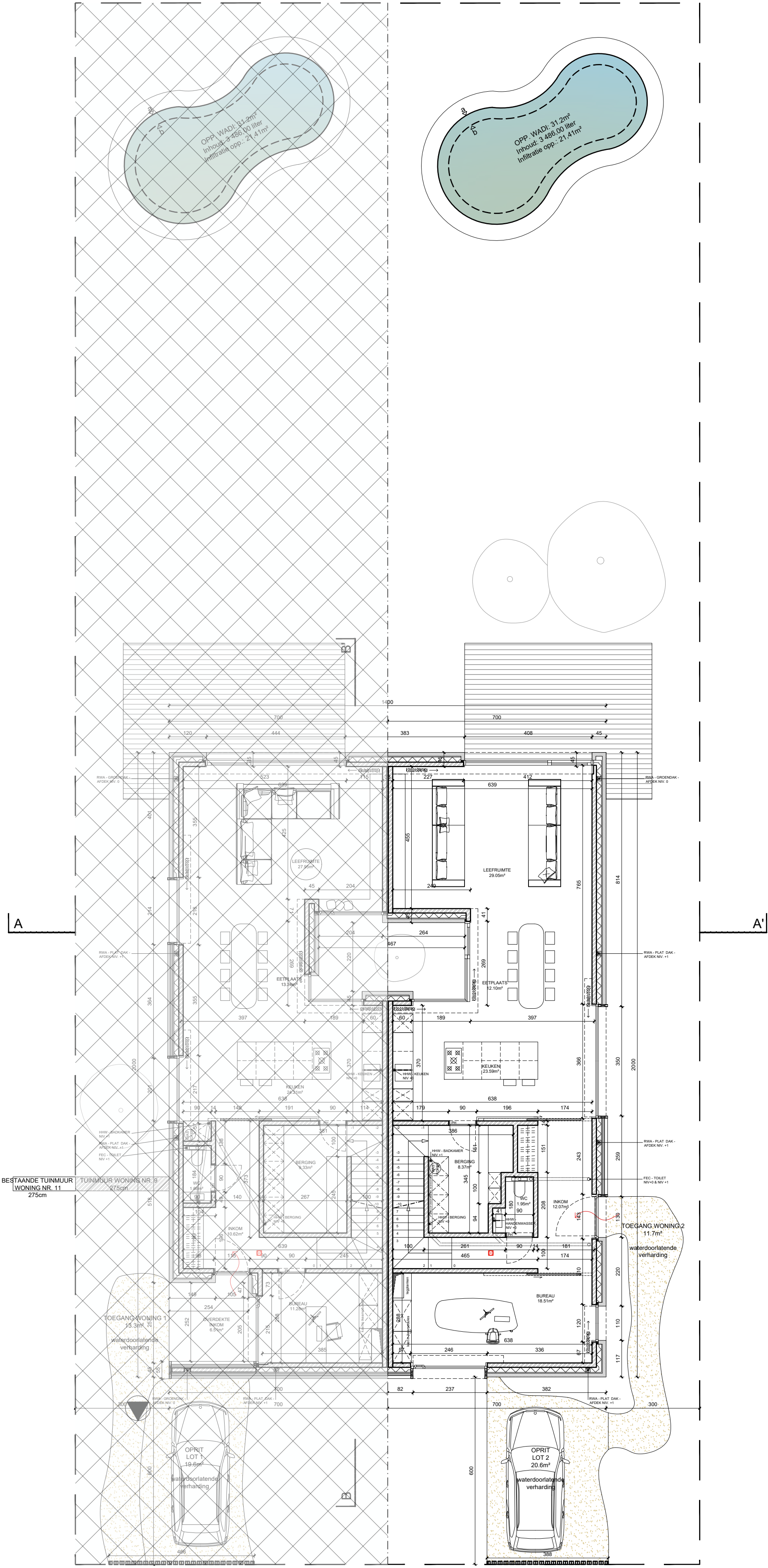
PLAN NIVEAU 0 - LOT 1 WONING - BRUTO OPP. : 128.6m² PLAN NIVEAU 0 - LOT 2 WONING - BRUTO OPP. : 134.6m² N
