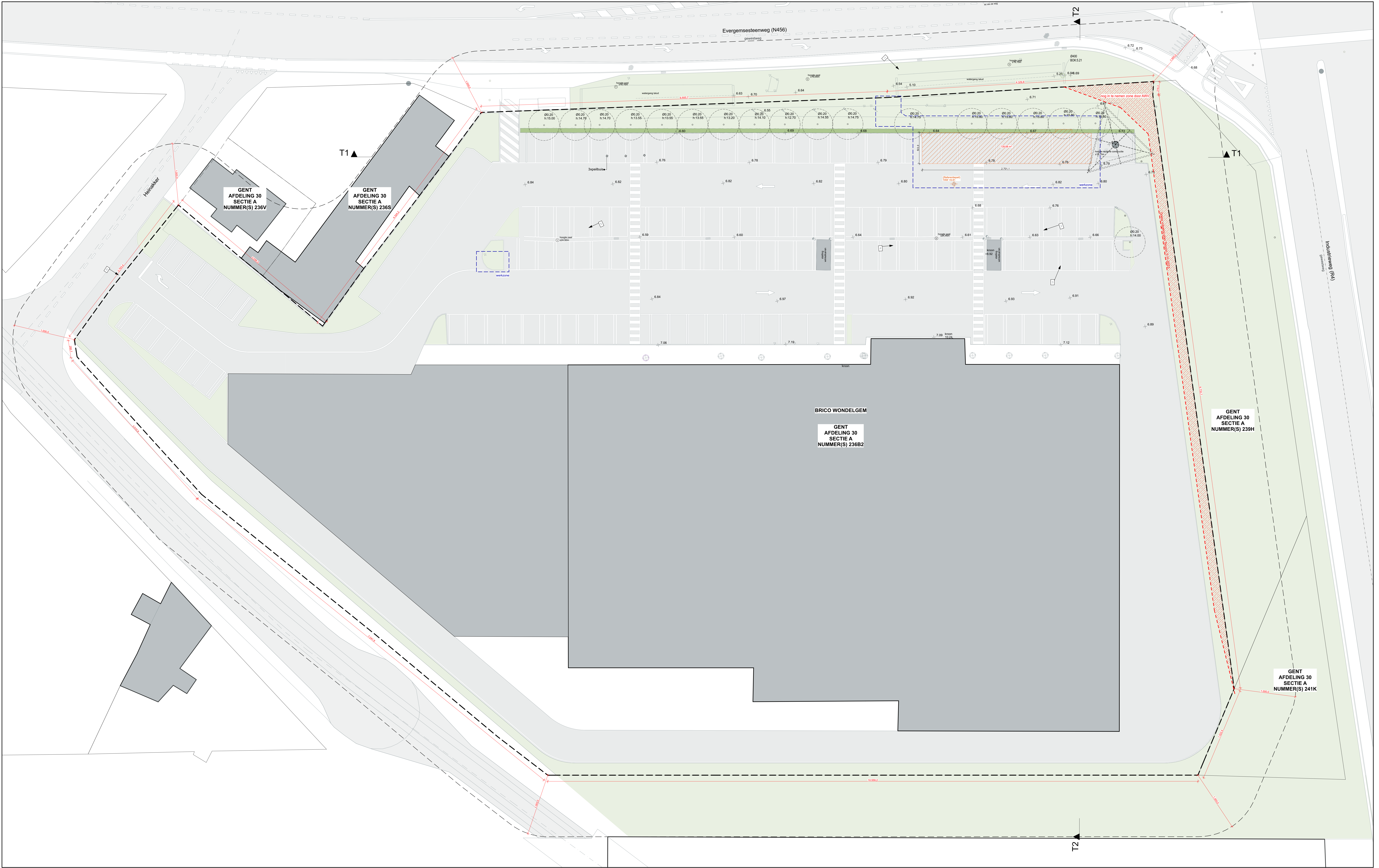
Implantingsplan BT
