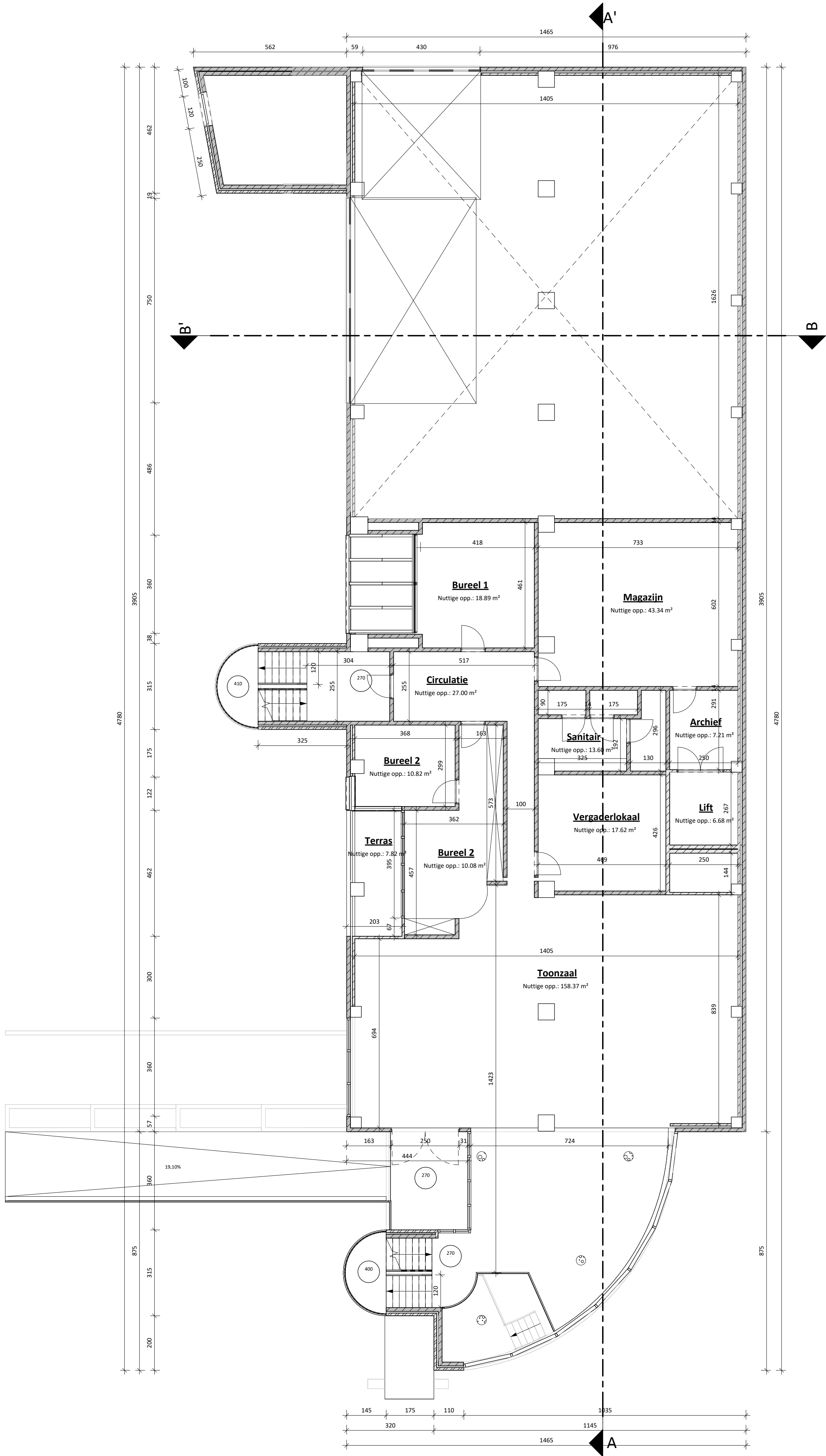
VT_Verdieping +1 | Vergunde toestand | 1 : 100
