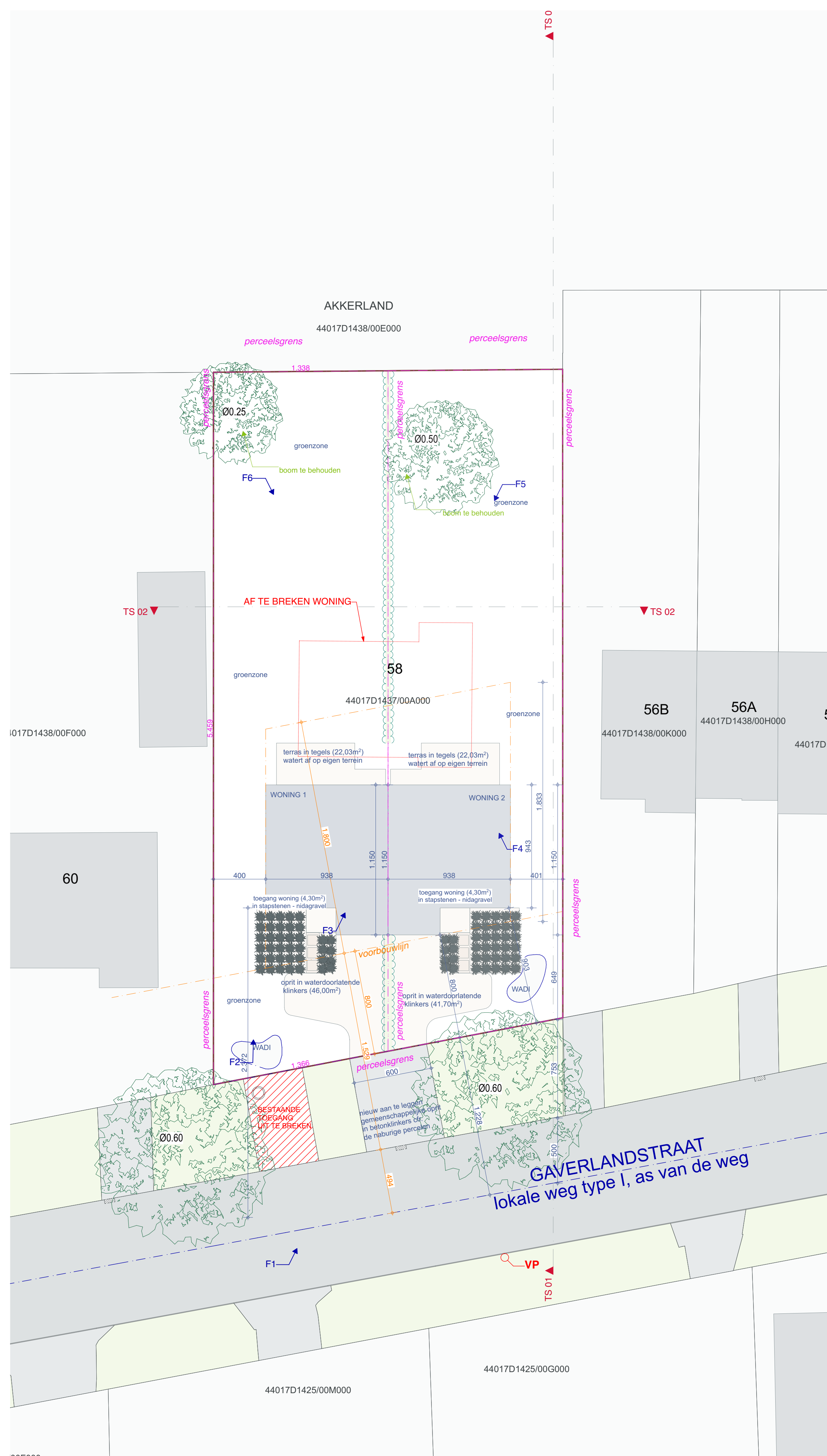
INPLANTINGSPLAN
