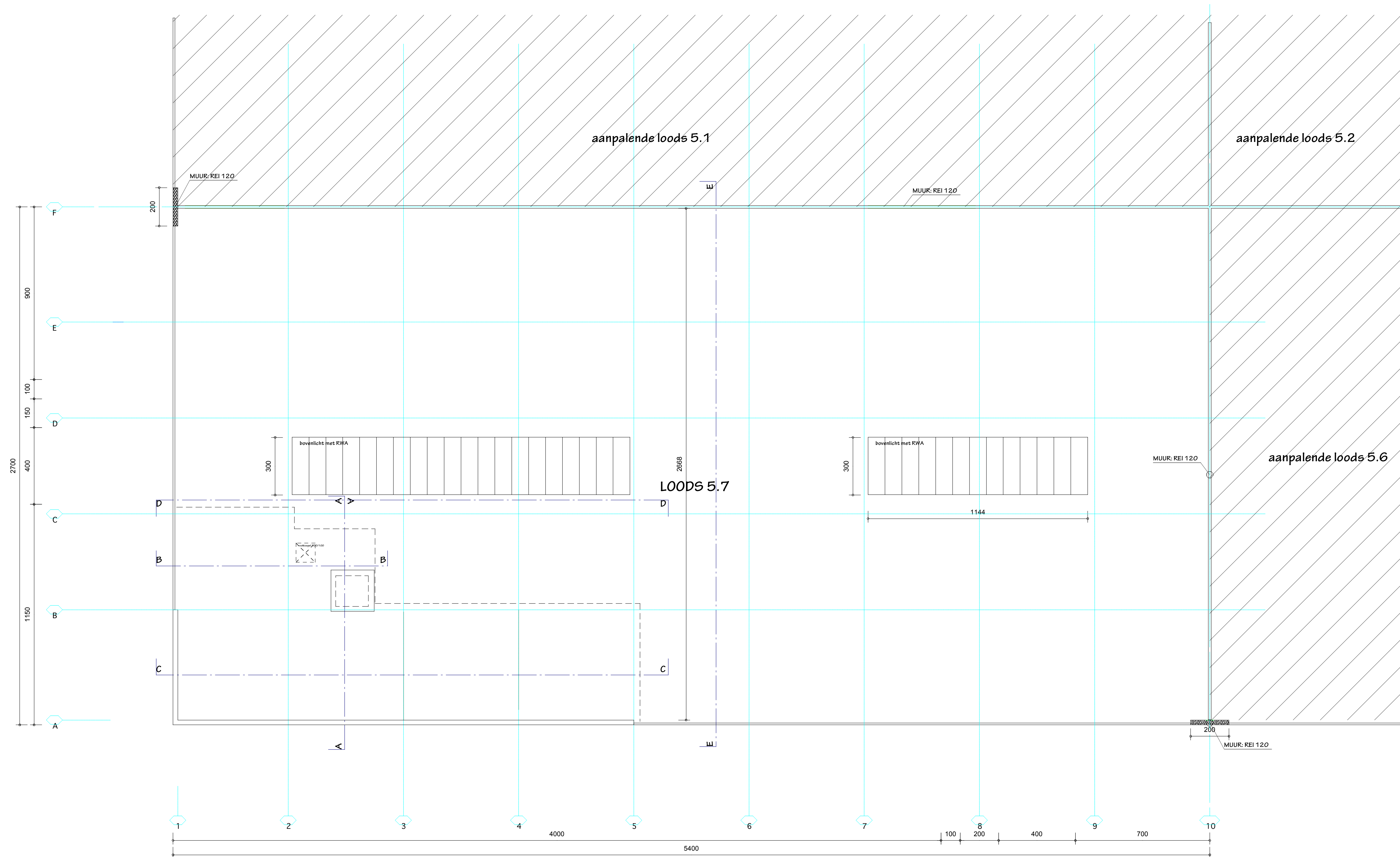
DAKENPLAN
