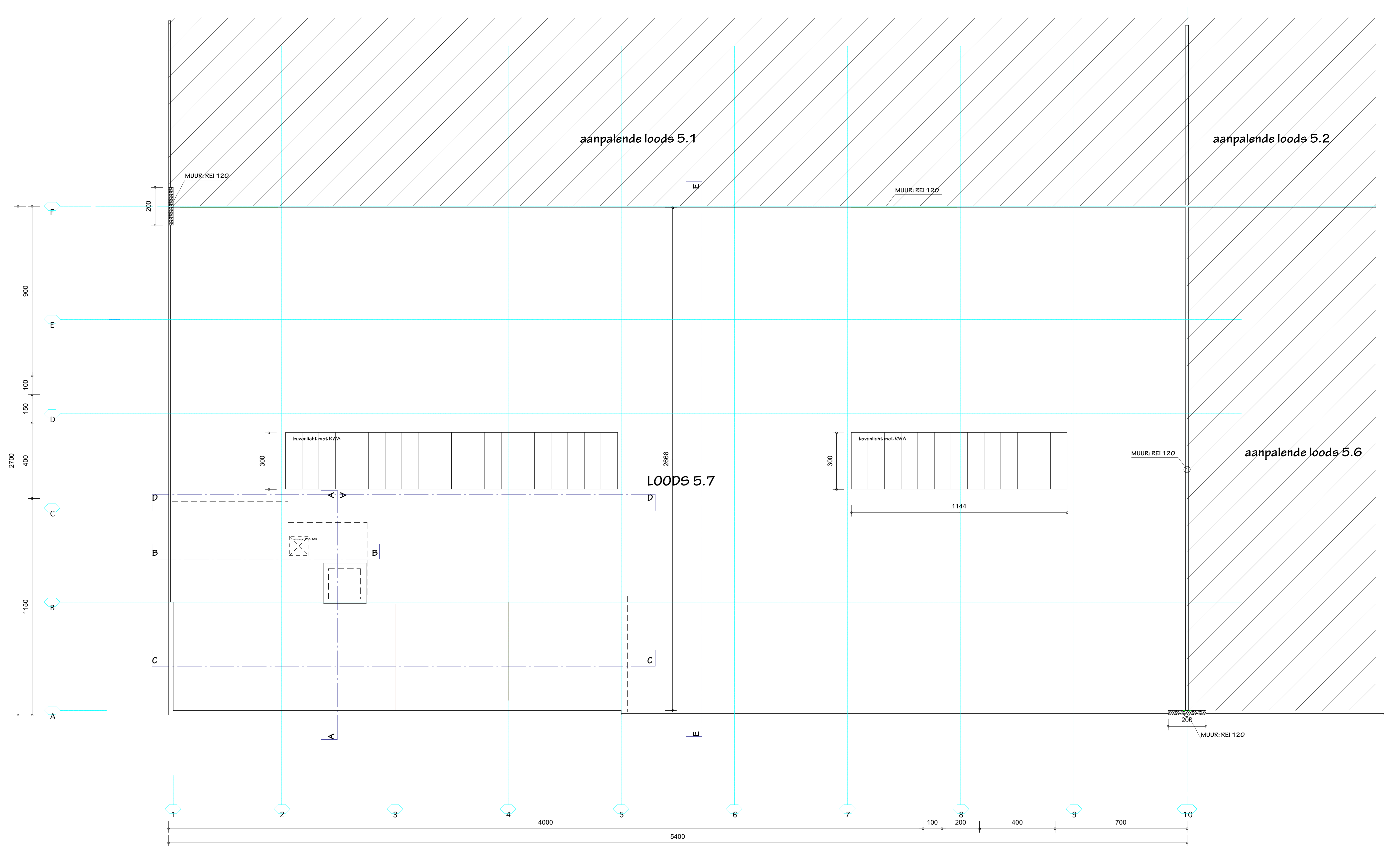
DAKENPLAN
