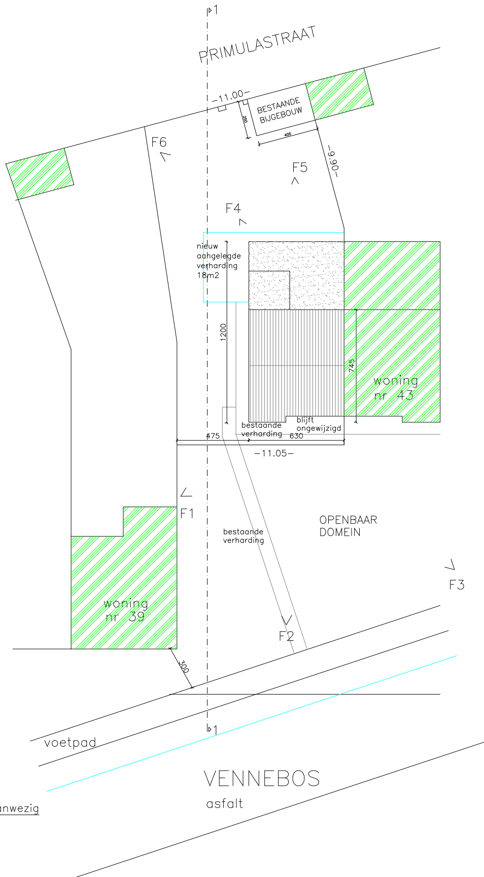
BA woning-I-N-1-inplantingsplan
