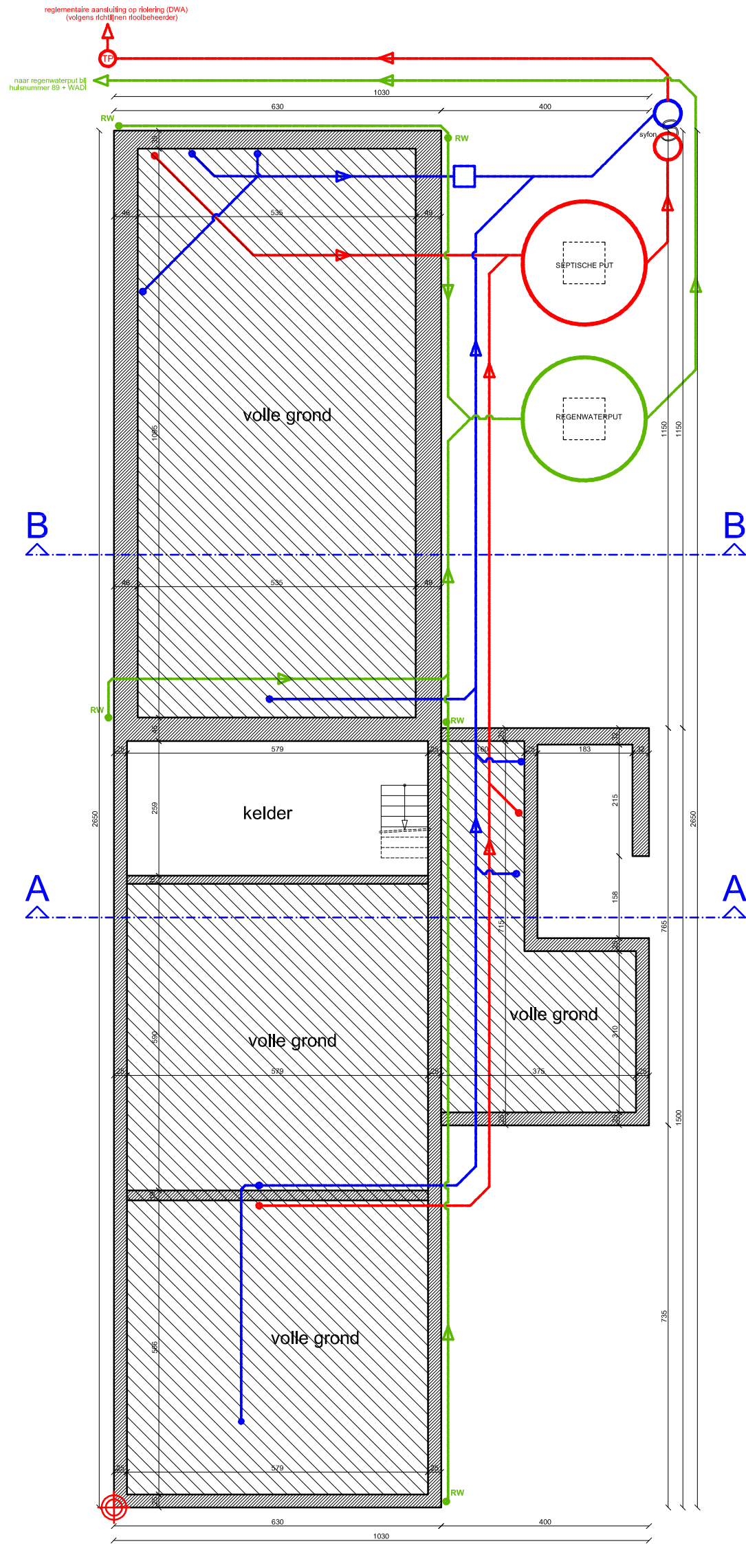
FUNDERING - VT
