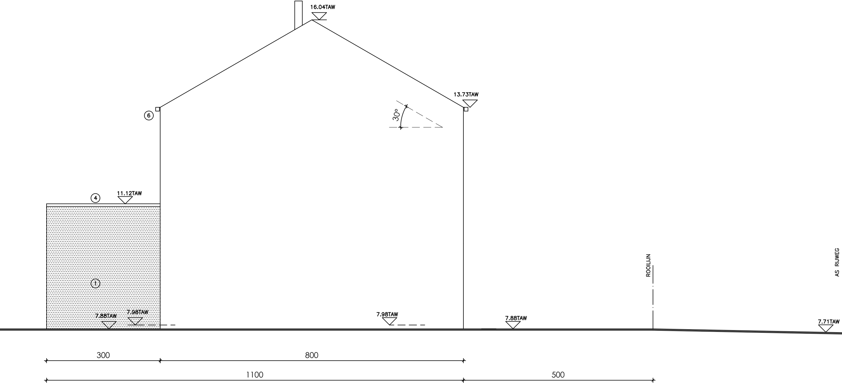
PROFIEL LOT 7
