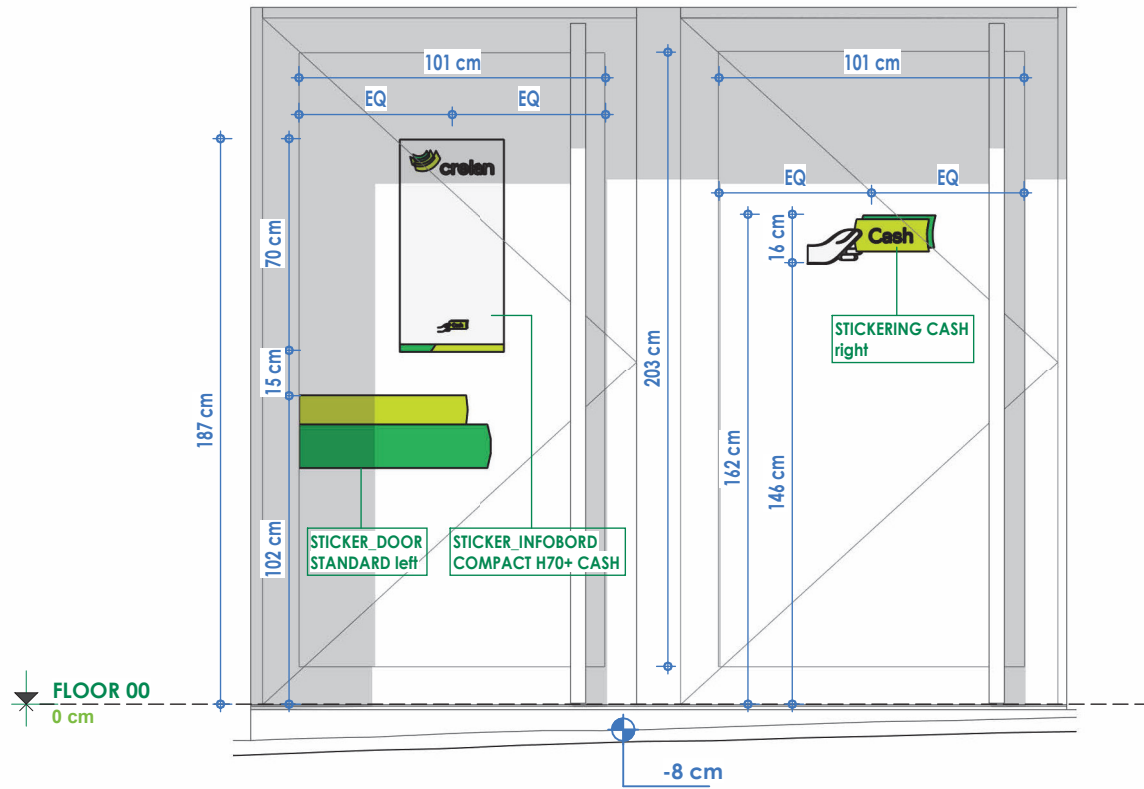
1 FACADE new - Callout 1 1 : 25
