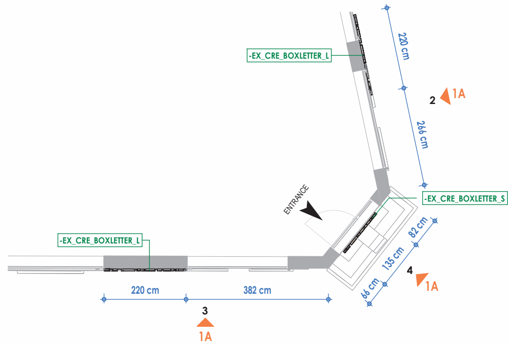
1 FLOOR PLAN existing 1 : 100
