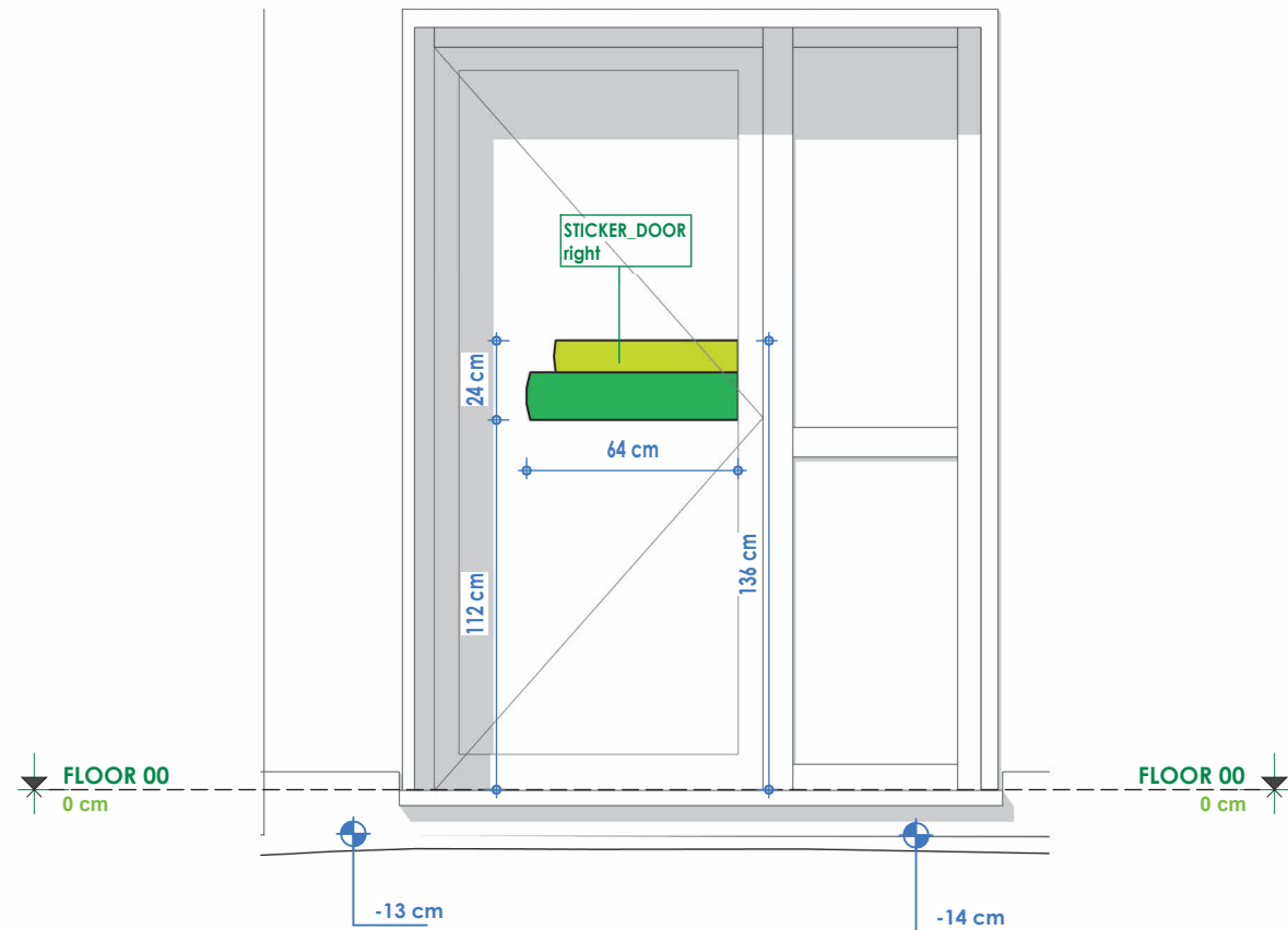
1 ELEVATION new - Entrance 1 : 25
