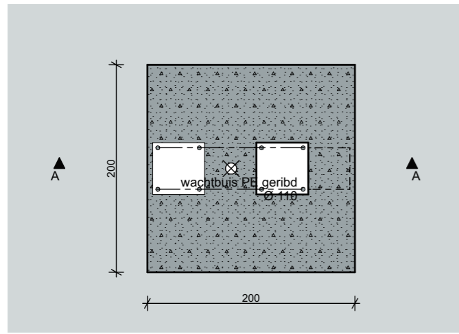
Funderingsplan
