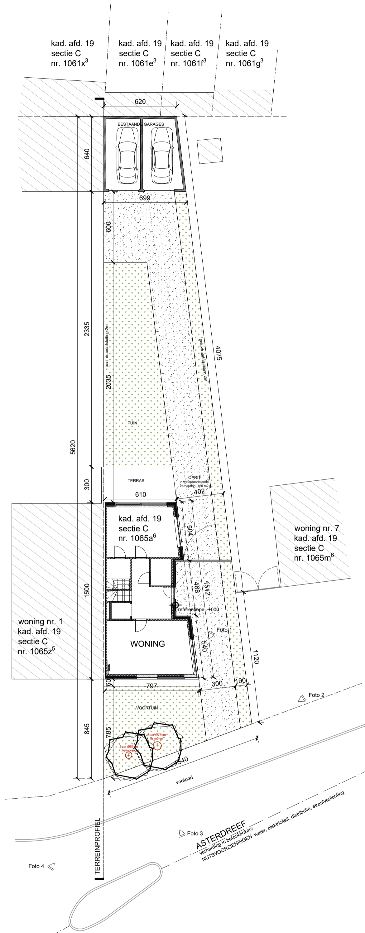
INPLANTINGSPLAN - 1/200
