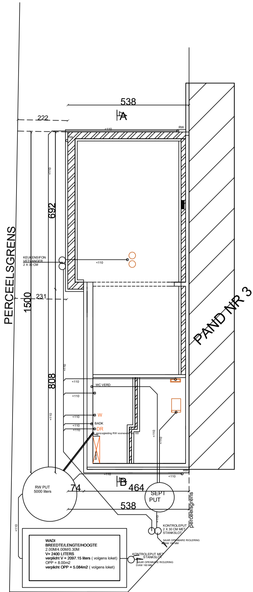
FUNDERINGS - RIOLERINGSPLAN 1/100
