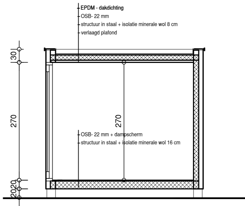
DOORSNED E A - A'
