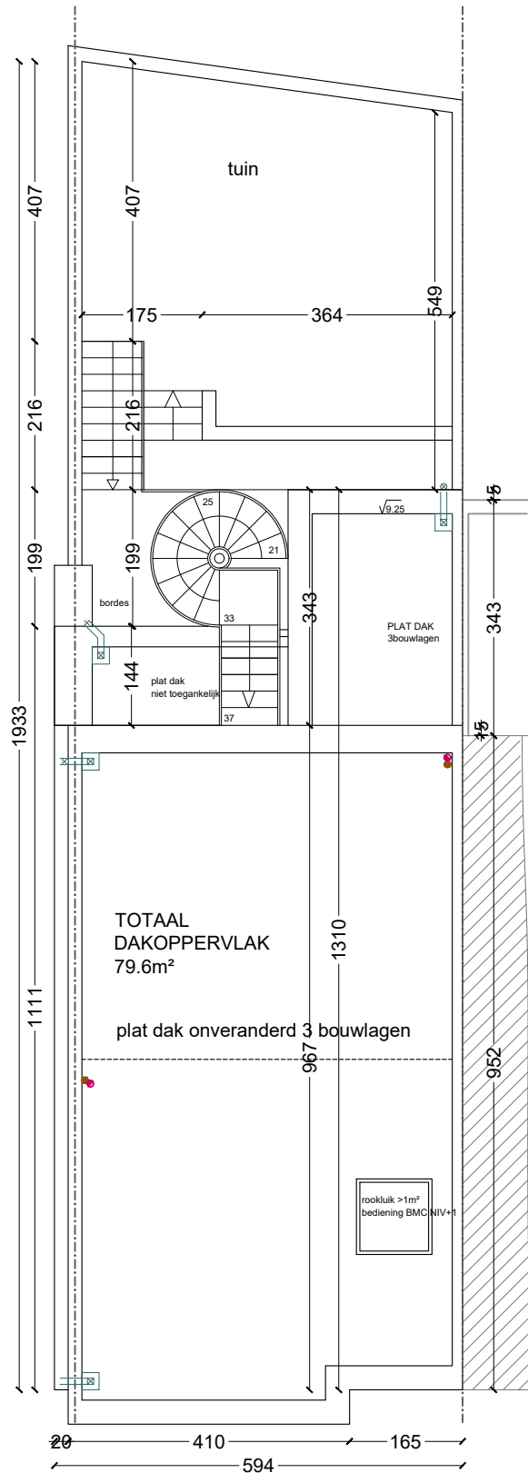
DAKPLAN
